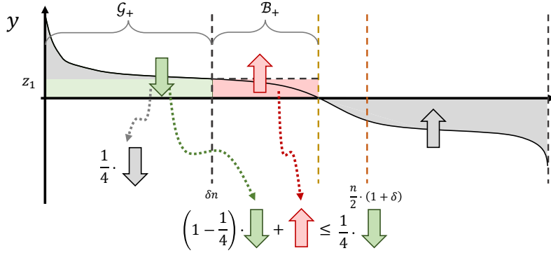
Figure 3.3: Case A.1: The dominant (positive) contribution of bins in \mathcal{B}_+ (shown in red) is counteracted by a fraction of the (negative) contribution term of the good bins \mathcal{G}_+ (shown in green). In grey, the dominant decrease terms for \mathcal{G}_+ and \mathcal{G}_- (which do not contribute to counteracting the increase).
