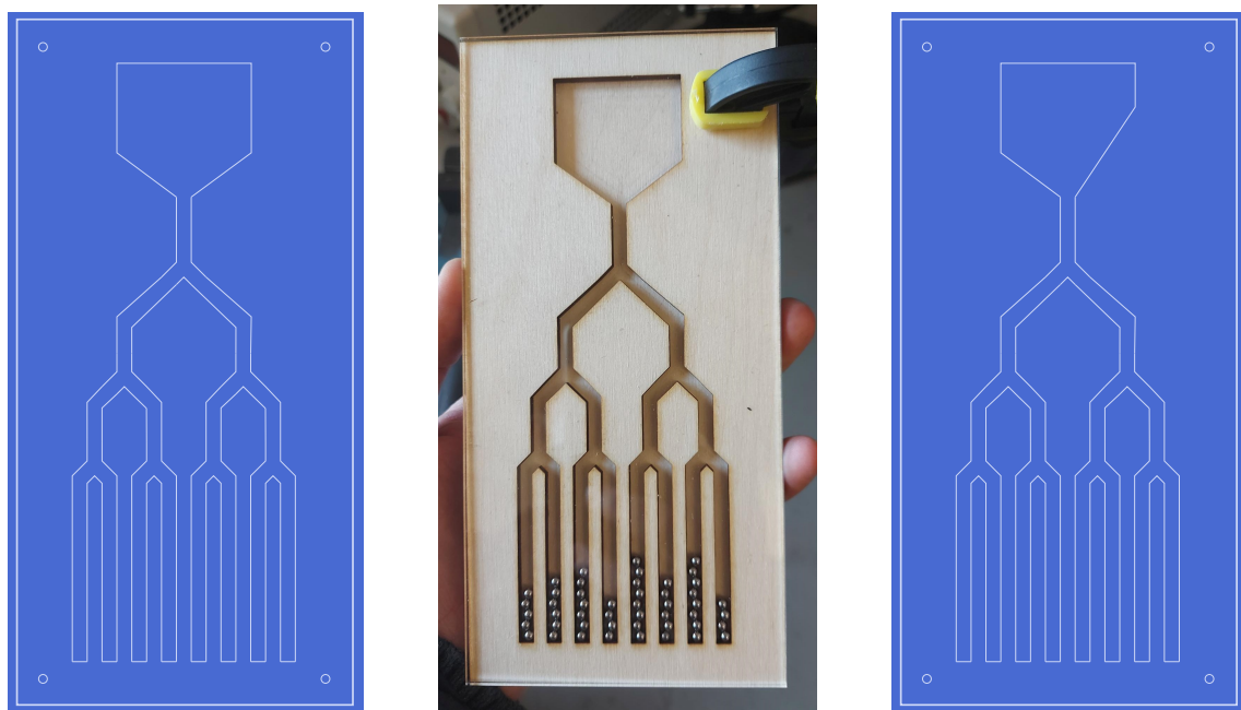
Figure 3.6: On the left is the blueprint for the ONE-CHOICE process, in the middle is the actual implementation of this blueprint and on the right is the blueprint of a modification that prevents balls being stuck in the top junction.
