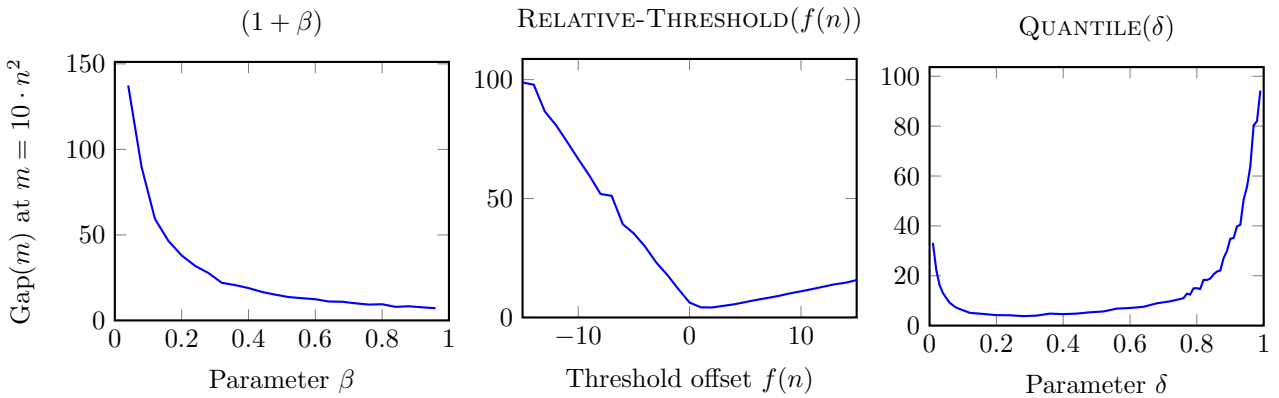
Figure E.3: The \text{Gap}(m) for n = 10^3 and m = 10^7 for different parameters of the (1 + beta) , RELATIVE-THRESHOLD(f(n)) and QUANTILE(delta) processes (15 repetitions).
