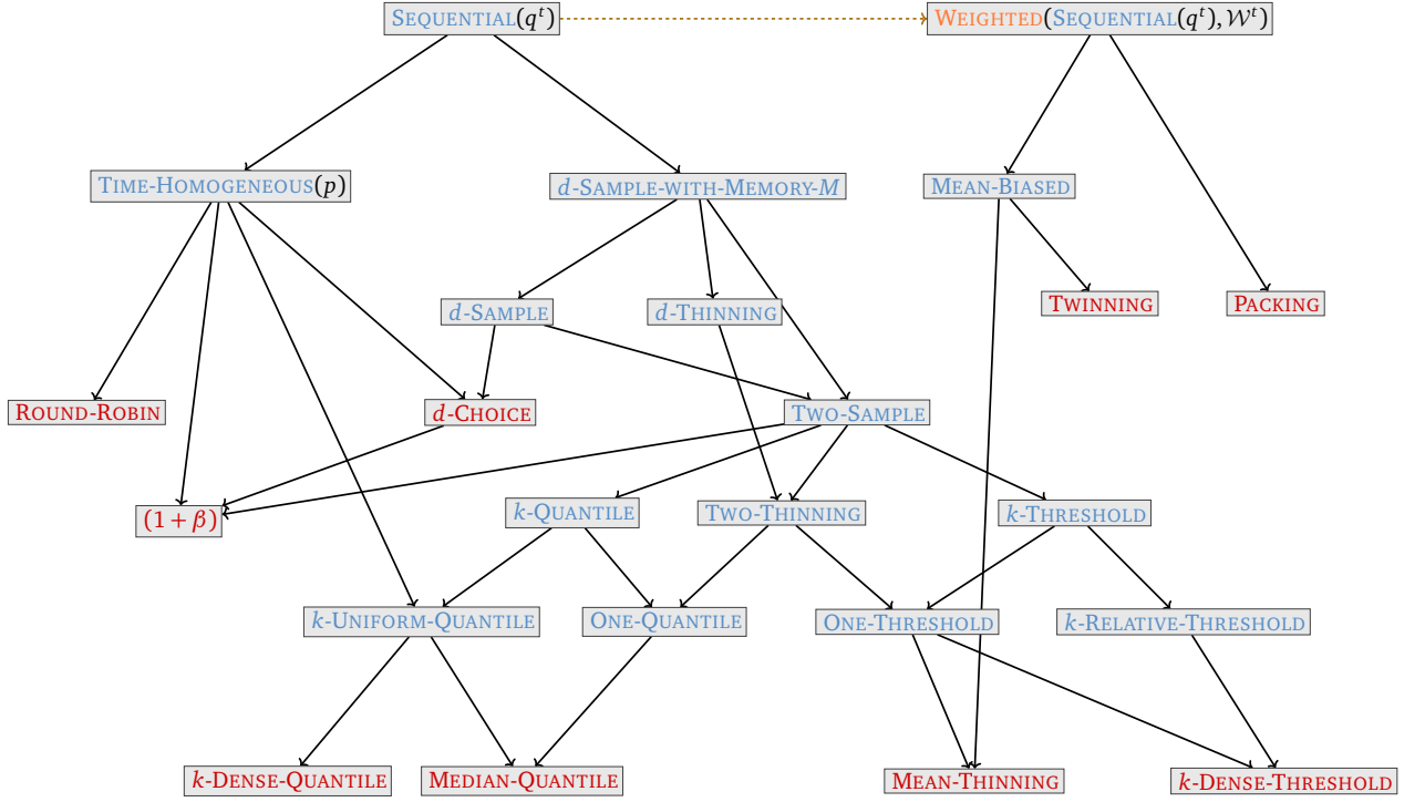
Figure 2.8: Hierarchy between some of processes and families of processes considered.
