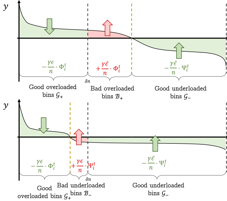
Figure 3.2: The two cases of bad bins ( \mathcal{B}_+ \neq \emptyset and \mathcal{B}_- \neq \emptyset respectively) in a load vector and their dominant terms in \Delta\bar{\Gamma} for each of the set of bins. The dominant terms that are decreasing are shown in green and the dominant terms that are increasing are shown in red.
