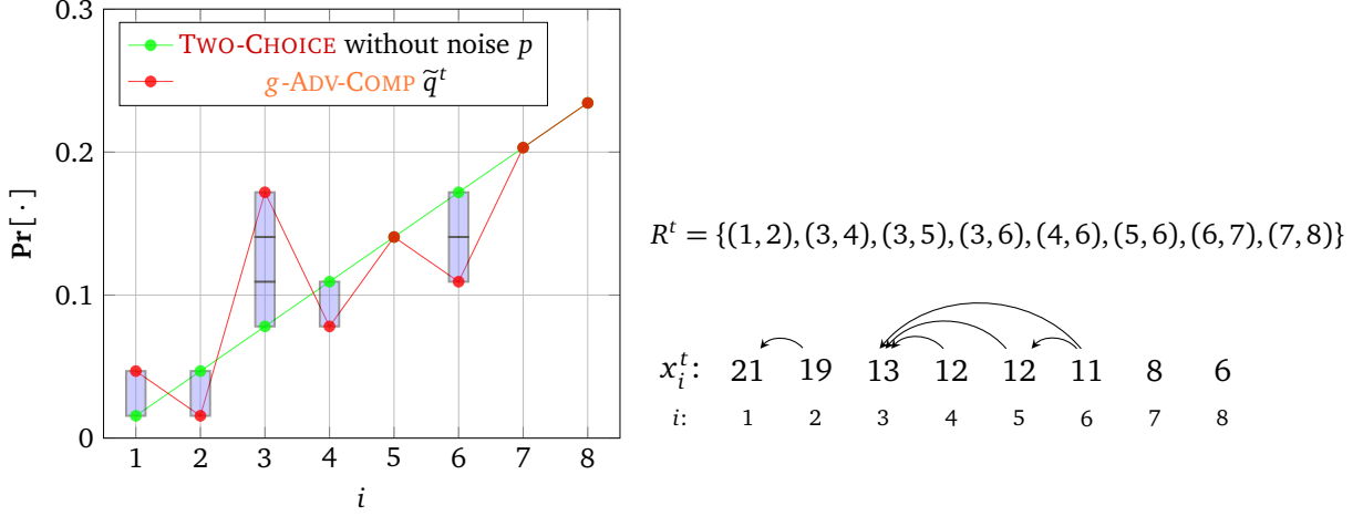
Figure 3.5: Illustration of the set R^t and the change in the sorted allocation vector from p to \tilde{q}^t , where n = 8 and g = 3 . In the example, each directed arrow moves a probability of \frac{2}{n^2} (indicated by the blue rectangles) from a bin j to a heavier bin i < j . Note that in this example, the adversary decides not to reverse some of the comparisons, e.g., between bins 7 and 8.
