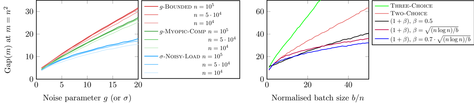
Figure E.1: The \text{Gap}(m) for n \in \{10^4, 5 \cdot 10^4, 10^5\} and m = n^2 for noisy settings of TWO-CHOICE and for various processes in the b-BATCHED setting (25 repetitions).
