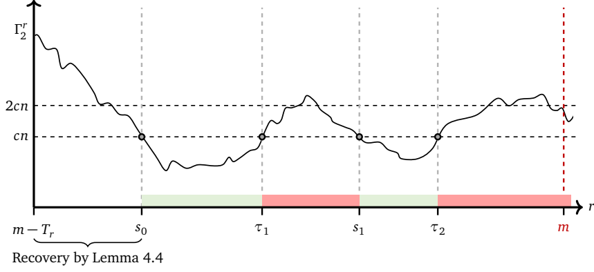
Figure 4.2: Green phases indicate steps where \Gamma_2^t is small and red phases indicate steps for which the potential is large and drops (in expectation). In Lemma 4.5, we show that \Gamma_2 \leq 3cn at every point within a red phase using a concentration inequality.
