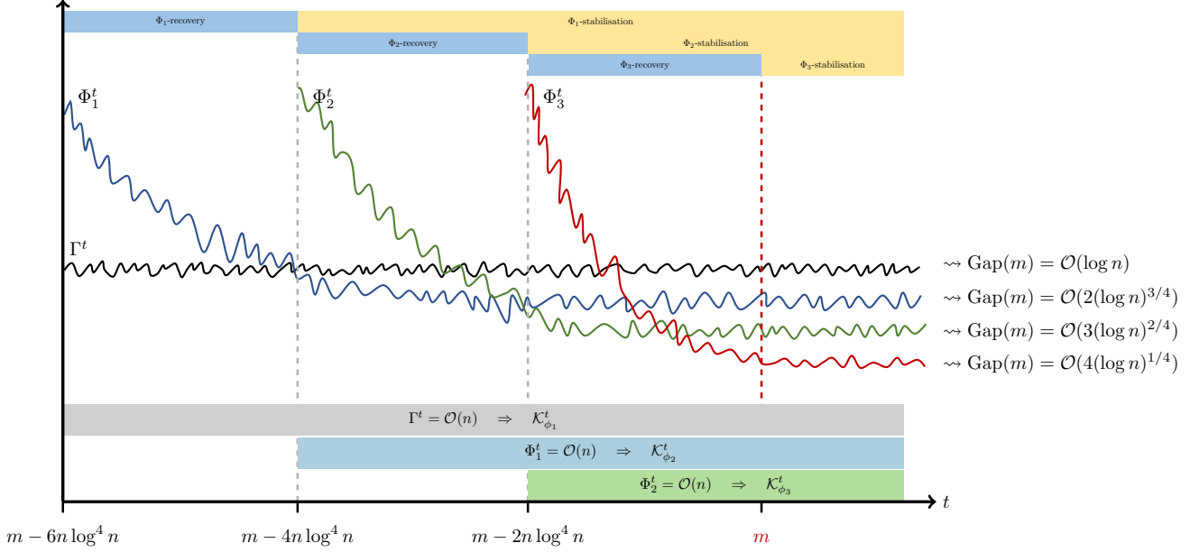
Figure 7.1: Layered induction for the k -DENSE-QUANTILE for k = 4 , showing that when the potential at layer j satisfies \Phi_j^t = \mathcal{O}(n) , the drop condition at layer j + 1 , i.e., \mathcal{K}_{\phi_{j+1}}^t is implied. Then, after a recovery phase the potential \Phi_{j+1} stabilises at \mathcal{O}(n) and implies a tighter bound on the gap.
